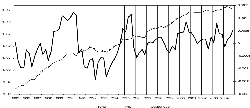
Figure 1. Trend/Cycle decomposition SVAR Model
